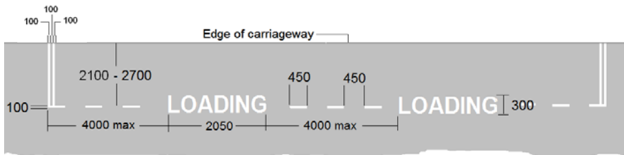
RRM 009: Loading Bay Markings
