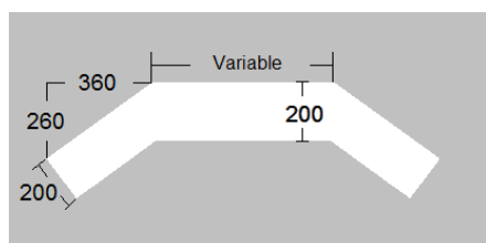
RRM 031 – Tram Stop Line
