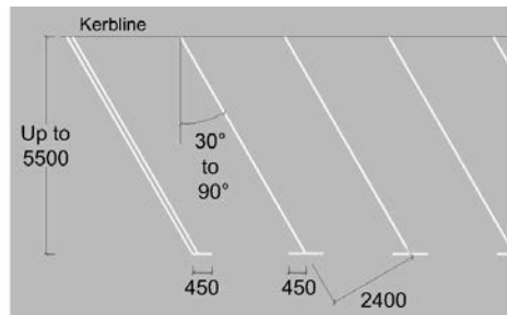
RRM 014: Angled Parking Bay Markings
