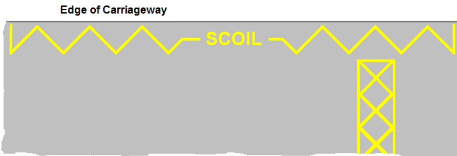
Figure 7.26: Combination of RRM 010 and M 121 Markings
