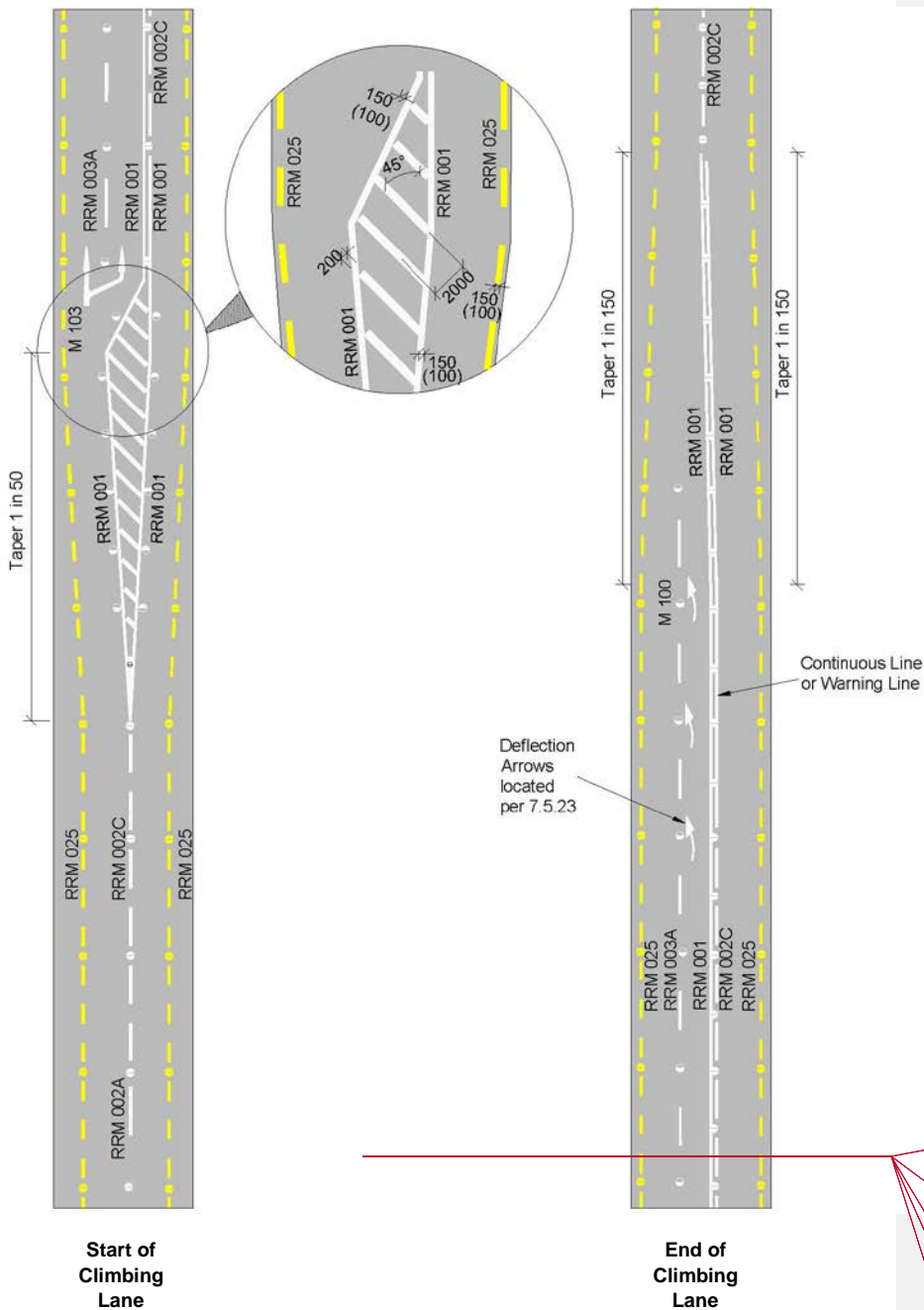
Figure 7.4: Longitudinal Lining for a Climbing Lane
