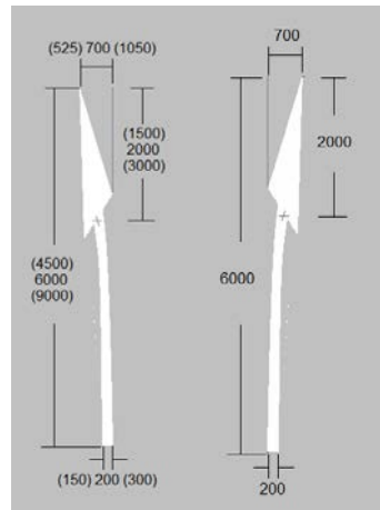
M 100 & M 101: Deflection Arrows
