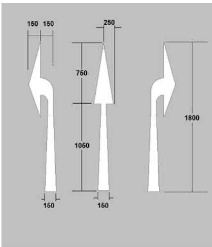
M 117 M 118 M 119 Cycle Track Direction Arrows
