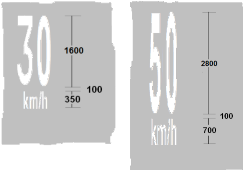
M 108: Speed Markings
