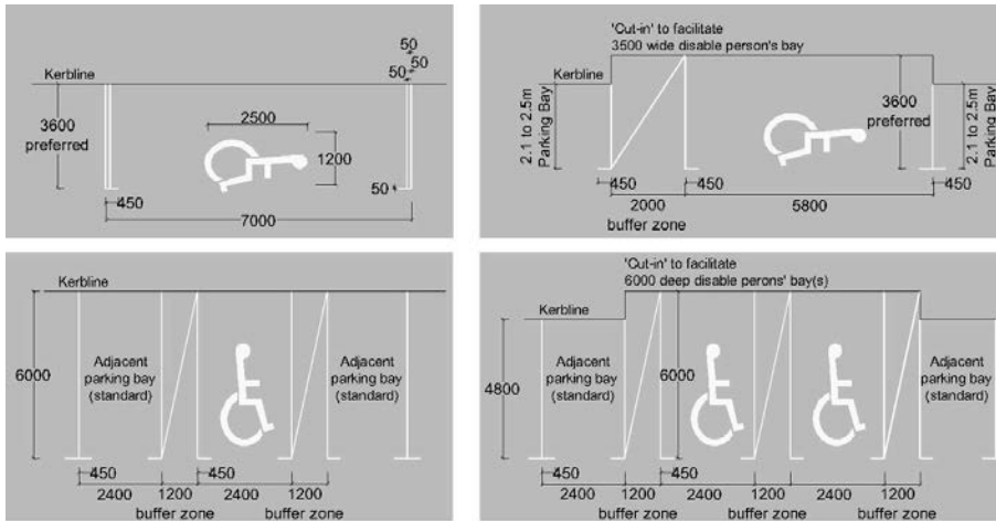
Figure 7.27: Typical Examples of Disabled Persons' Parking Bays
