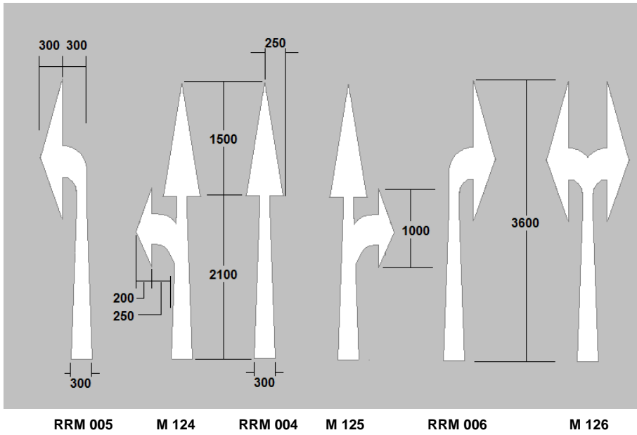
Figure 7.24: Lane Indication Arrows ( \leq 60\text{km/h} )
