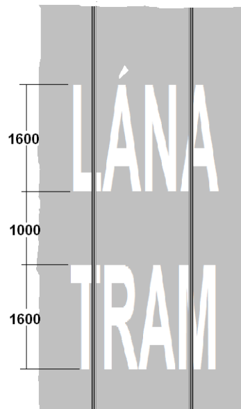
M 109: LÁNA TRAM Worded Marking
