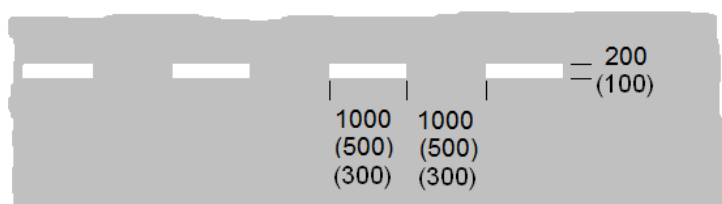
RRM 018 – YIELD Line
