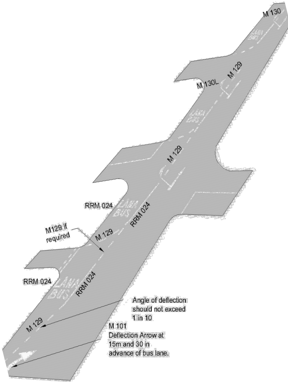
Figure 7.32: Typical Road Markings for a With-Flow Bus Lane
