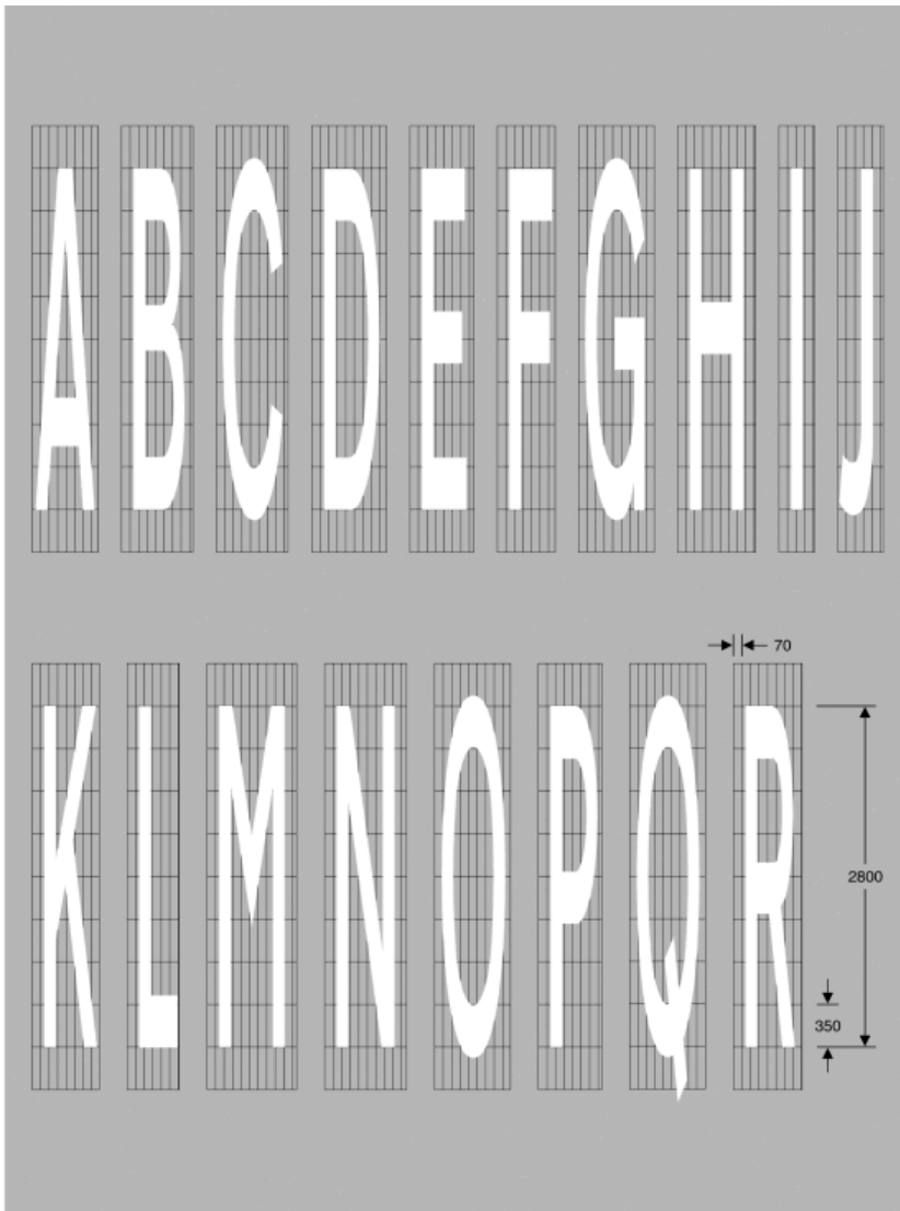
Figure 7.62: 2800mm Elongated Font
