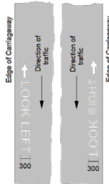
M 107: LOOK LEFT/RIGHT Marking
