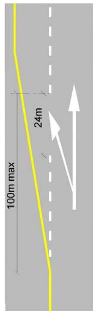
Diverge Lane Marking discontinued when the gap is 100m max in length or 2.5m from the taper.
