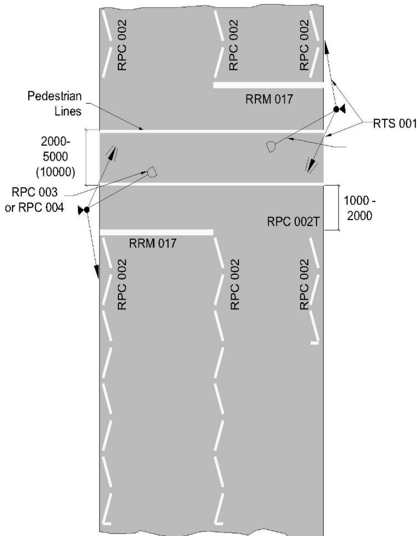
Figure 7.55: Signalised Pedestrian Crossing with RPC 002
