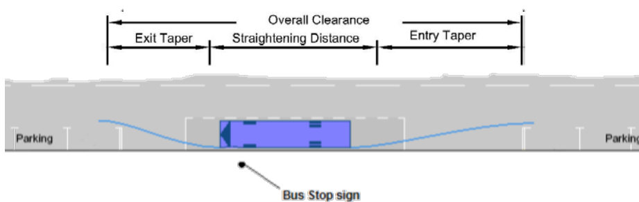
Figure 7.28: Clearance at Bus Stop Required for Parallel Docking (12m Rigid Bus)
