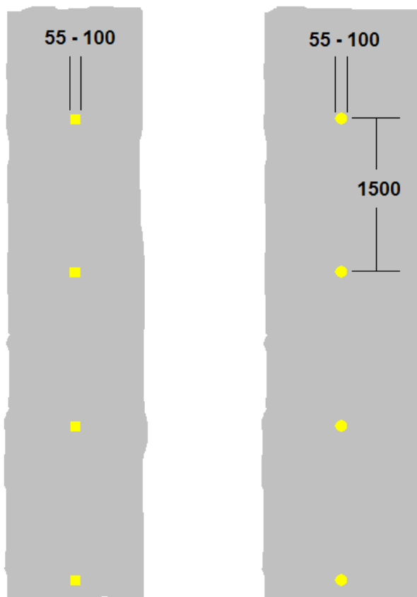
M 110: Light Rail Swept Path Marking
