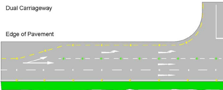
Figure 7.38: Permitted Edge Line Arrangements on Approach to a Junction on an All Purpose Road (Similar Arrangements on a Single Carriageway)
