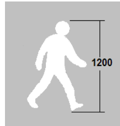
M 111 – Pedestrian Symbol
