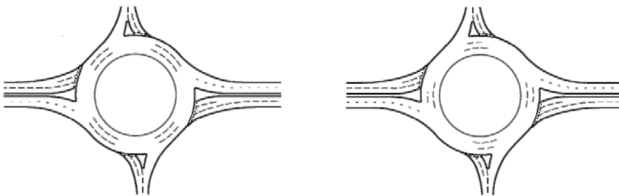
Figure 7.46: Partial Concentric Circulatory Markings
