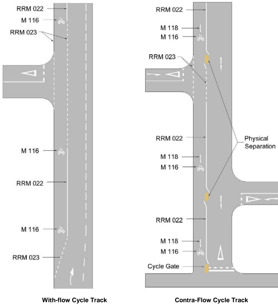
Figure 7.34: Sample Cycle Track Layouts
