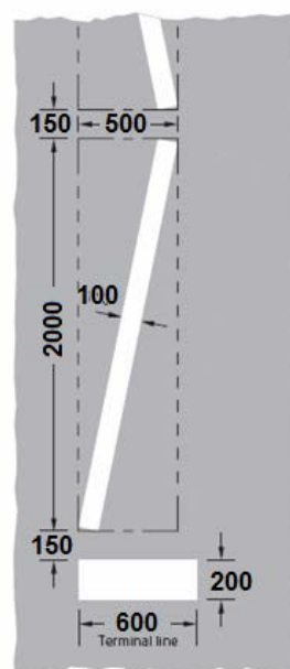
RPC 002: Zigzag and Terminal Line
