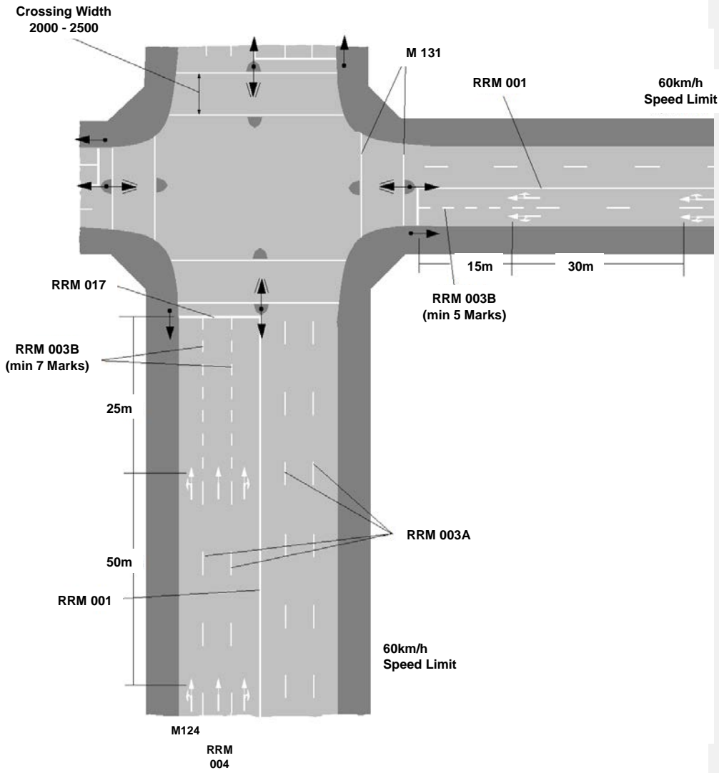
Figure 7.43: Markings at an Urban Signal-Controlled Junction
