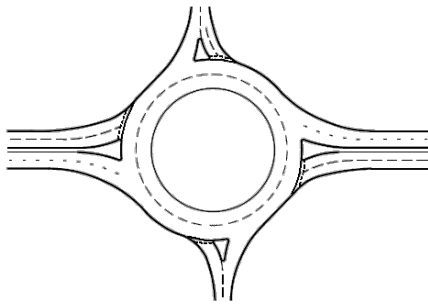
Figure 7.45: Concentric Circulatory Markings
