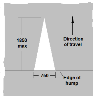
M 112 Traffic Calming Triangle
