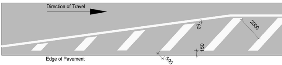
Diagonal Hatched Marking for Use on Offside of Motorways and High-Quality Dual Carriageways
