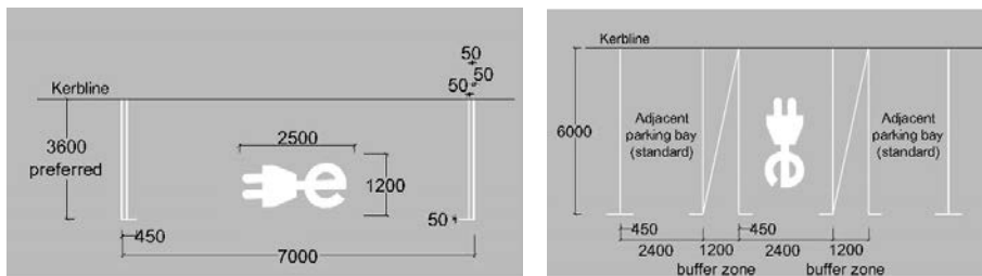
RRM 034: Electric Vehicle Recharging Bay Markings
