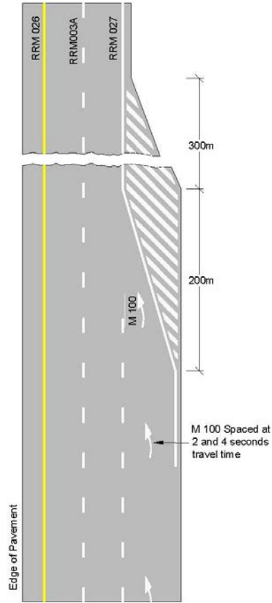
Figure 7.21: Example of Motorway Lane Reduction Markings
