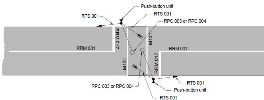
Figure 7.53: Signalised Pedestrian Crossing
