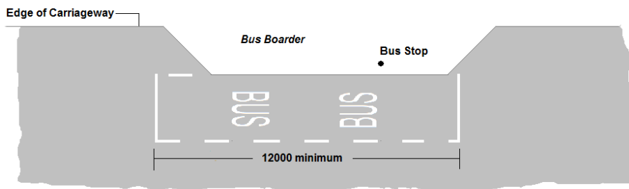
Figure 7.29: Bus Stop Marking at a Bus Boarder
