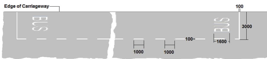
RRM 030: Bus Stop Markings
