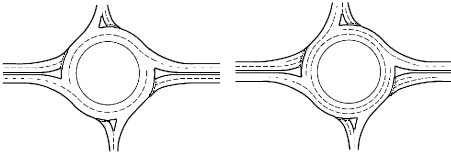
Figure 7.47: Concentric Spiral Circulatory Markings
