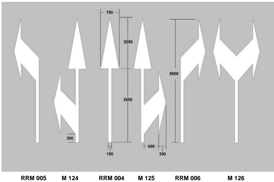
Figure 7.25: Lane Indication Arrows ( > 60\text{km/h} )
