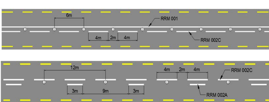
Figure 7.2(b): Double Line System
