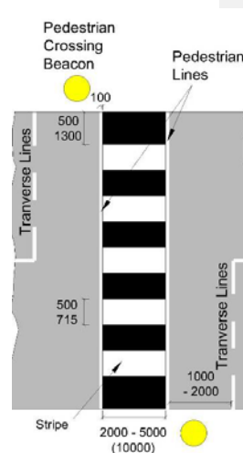
RPC 001: Zebra Crossing
