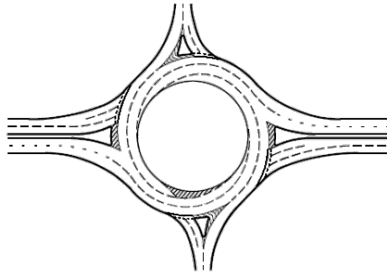
Figure 7.48: Spiral Circulatory Markings
