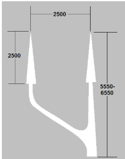
M 130: Double-headed Bus Lane Ends Arrow
