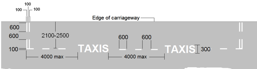
RRM 029: Taxi Stand Markings
