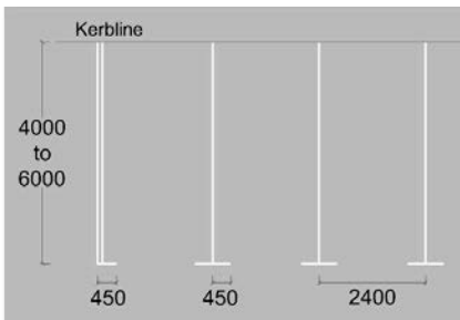
RRM 013: Perpendicular Parking Bay Markings
