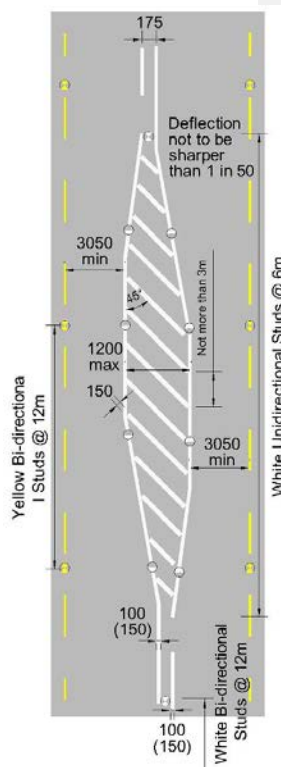
M104 Ghost Island at Crest
