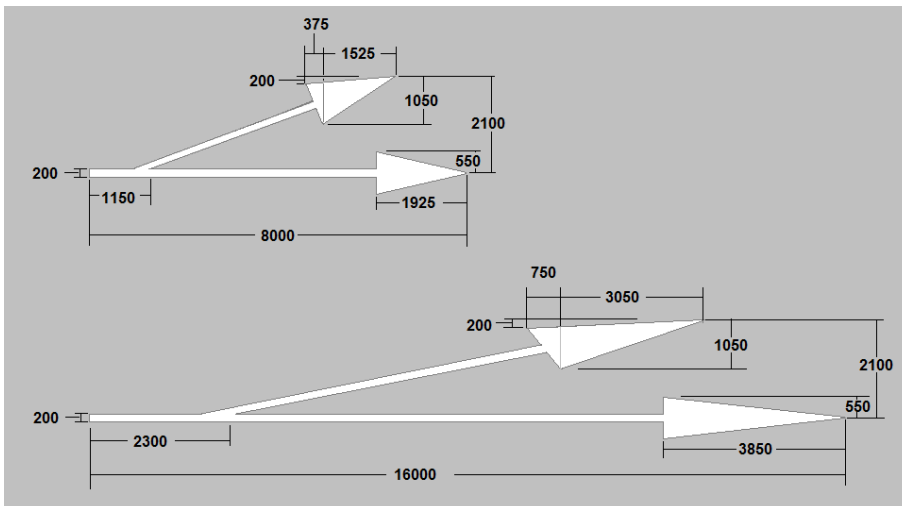
M 102: Bifurcation Arrows
