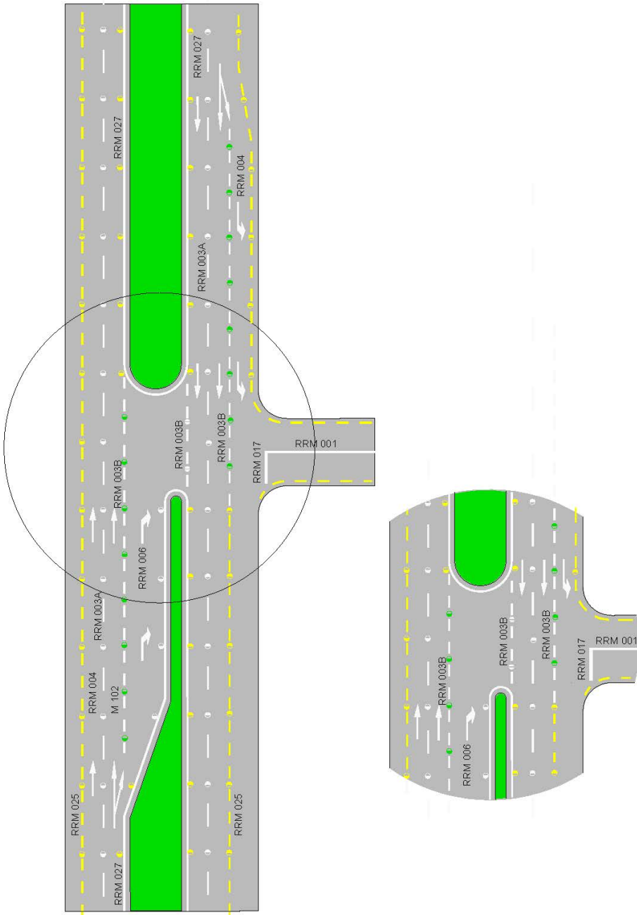
Figure 7.42: Dual Carriageway with Right Turn Lane
