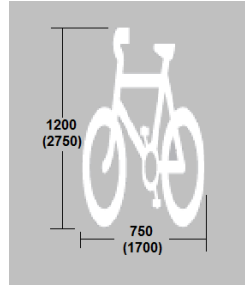
M 116 – Cycle Symbol
