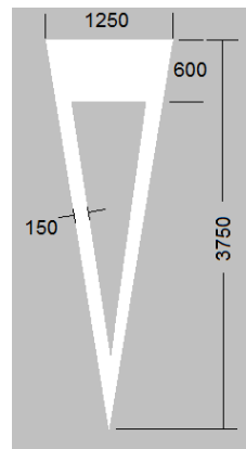
M 115: Triangular Yield Marking
