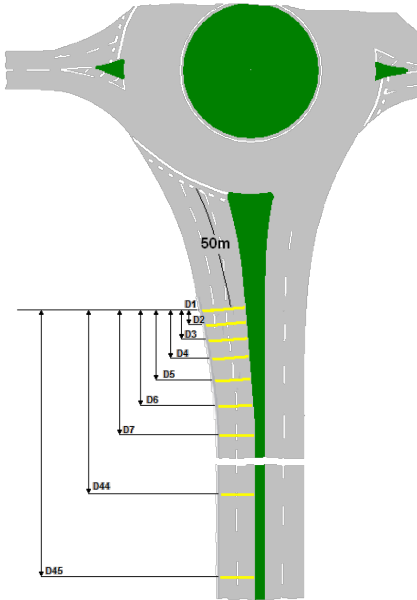
Figure 7.58: Yellow Bar Markings on Approach to Roundabout
