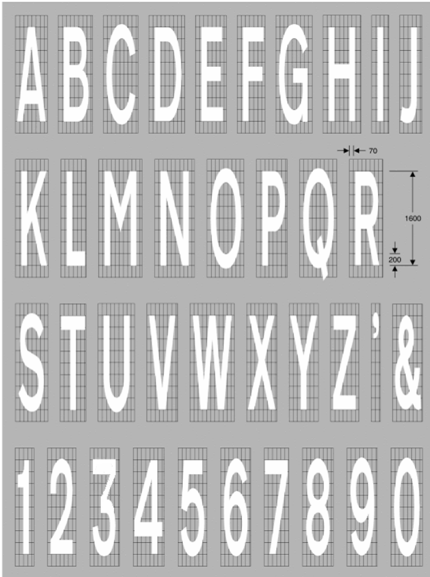
Figure 7.61: 1600mm Elongated Font
