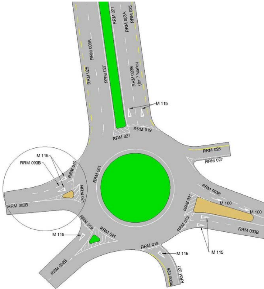
Figure 7.44: Markings at a Normal Roundabout
