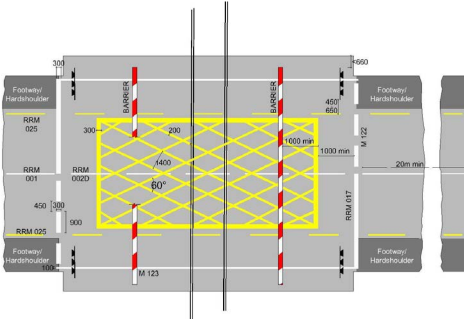
Figure 7.51: Markings at a Level Crossing
