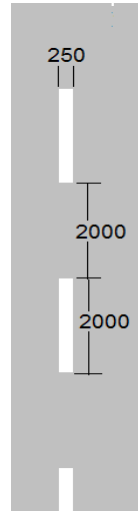
RRM 028: Merge/Diverge Lane Line
