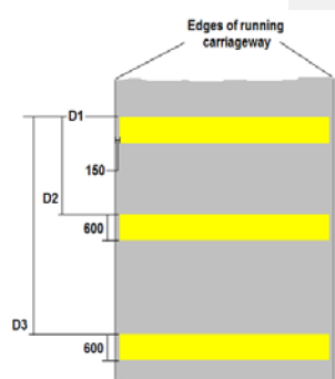
M 113: Yellow Bar Markings
