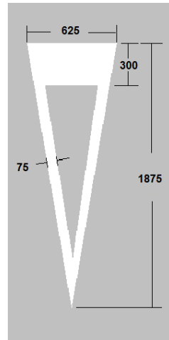
M115C Cycle Track Yield Marking
