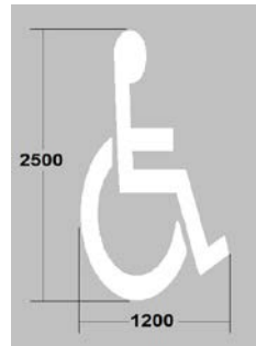
RRM 015: Disabled Persons' Parking Bay Symbol
