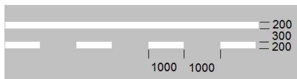
RRM 019 – No Entry Line
